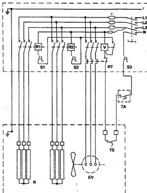
Quadro comando Terminal board 380V / 50Hz + N
